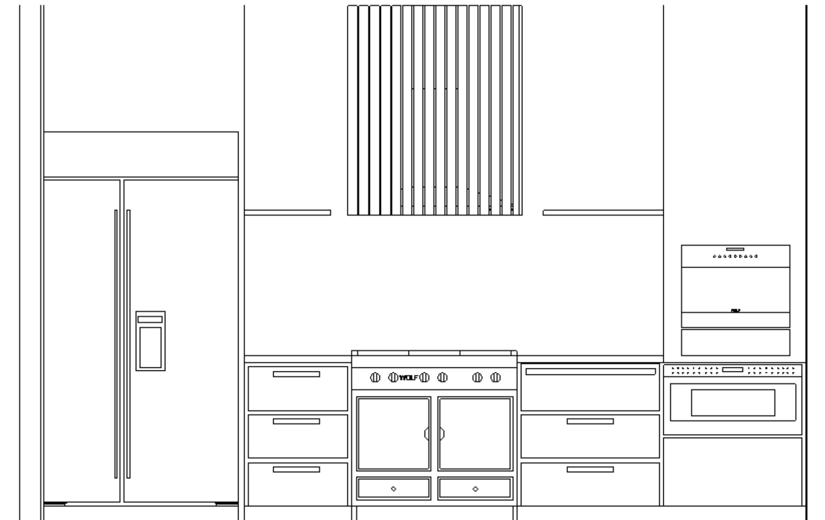
KITCHEN ELEVATION
